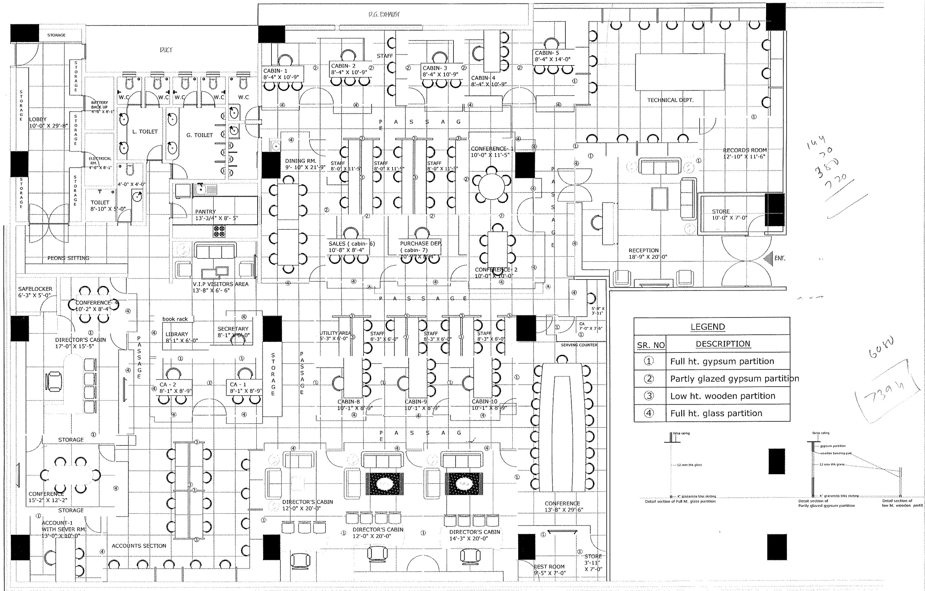
REVISED FULL & FINAL FURNITURE LAYOUT OF OFFICE AREA FOR S.M.C. AT THANE , SCALE: FIT TO SCALE. DATE: 01.12.2010
