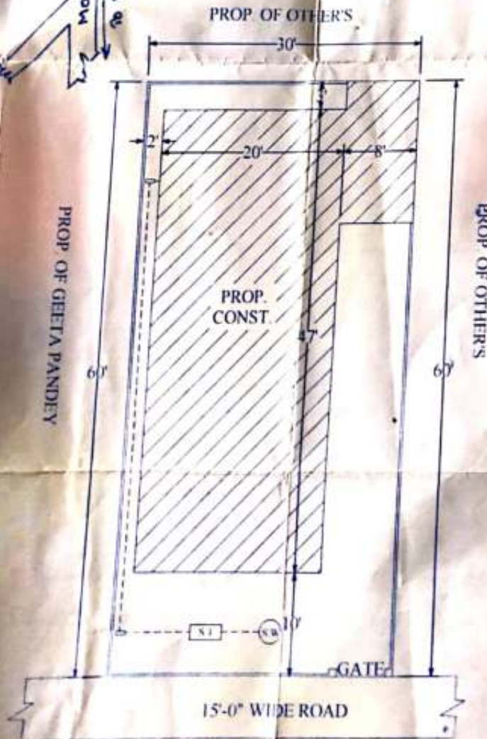
SITE PLAN
