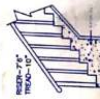
STAIR DETAIL
