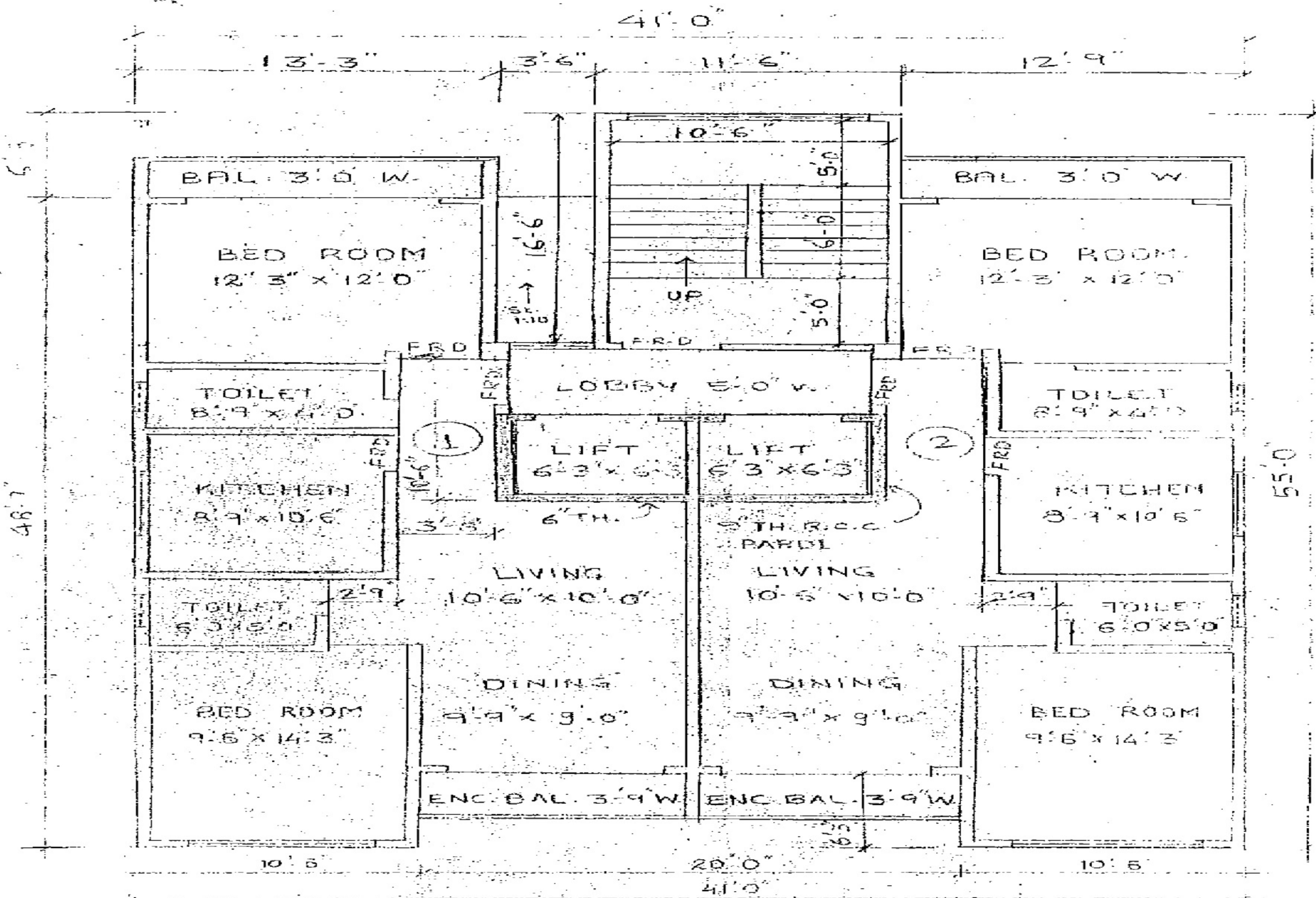
TYPICAL FLOOR PLAN (1 st TO 7 th AND 9 th TO 14 th )
