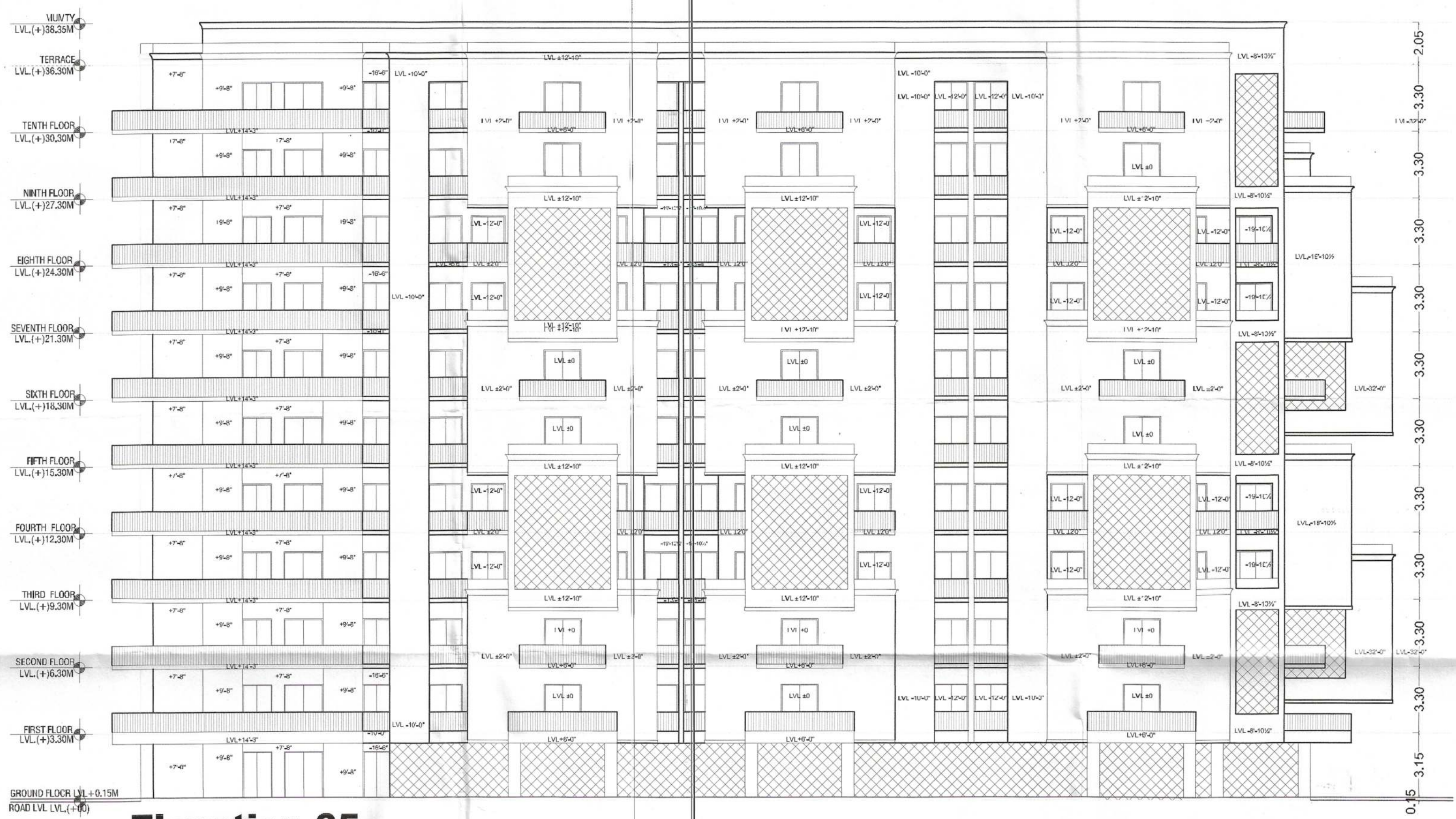
Elevation-05
