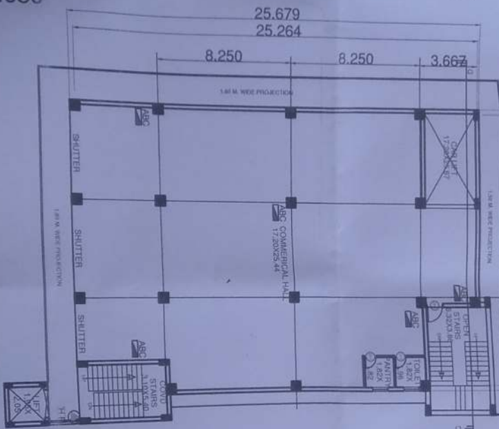
1st, 11nd, 111rd, 1Vth, FLOOR PLAN
