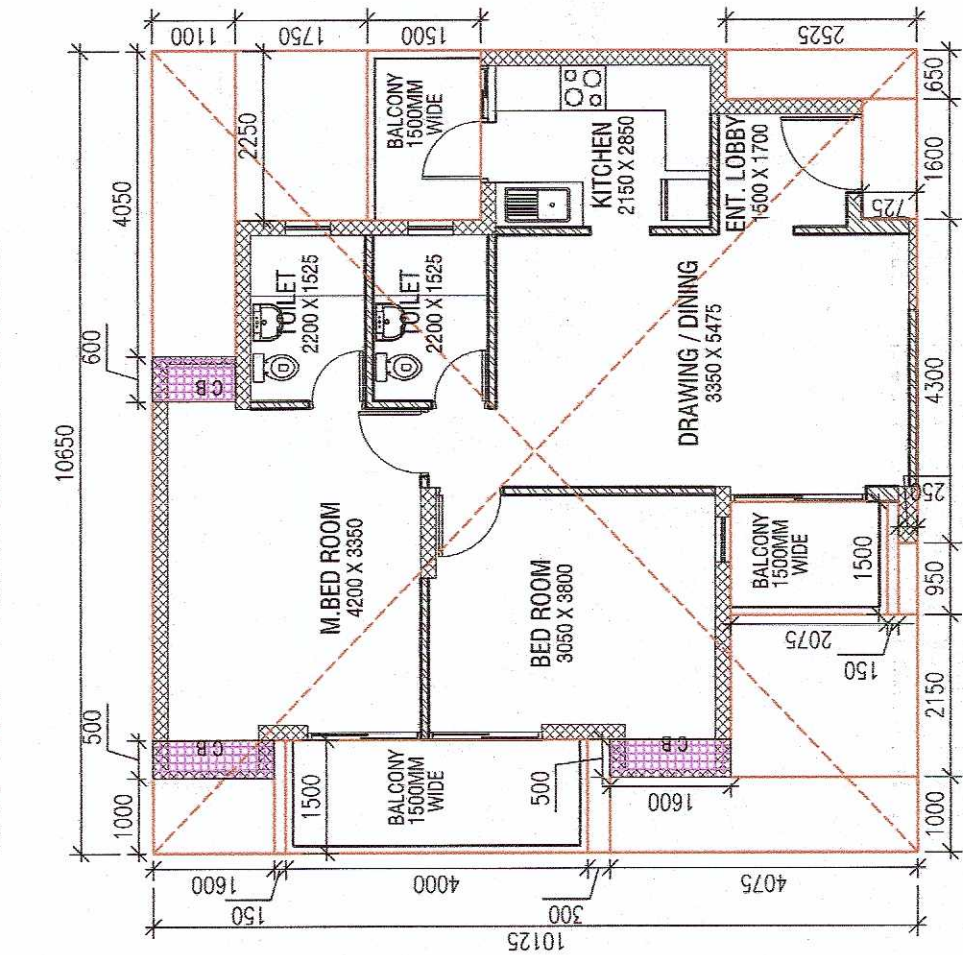
UNIT TYPE - 1 : 2BED ROOM +2TOILET
