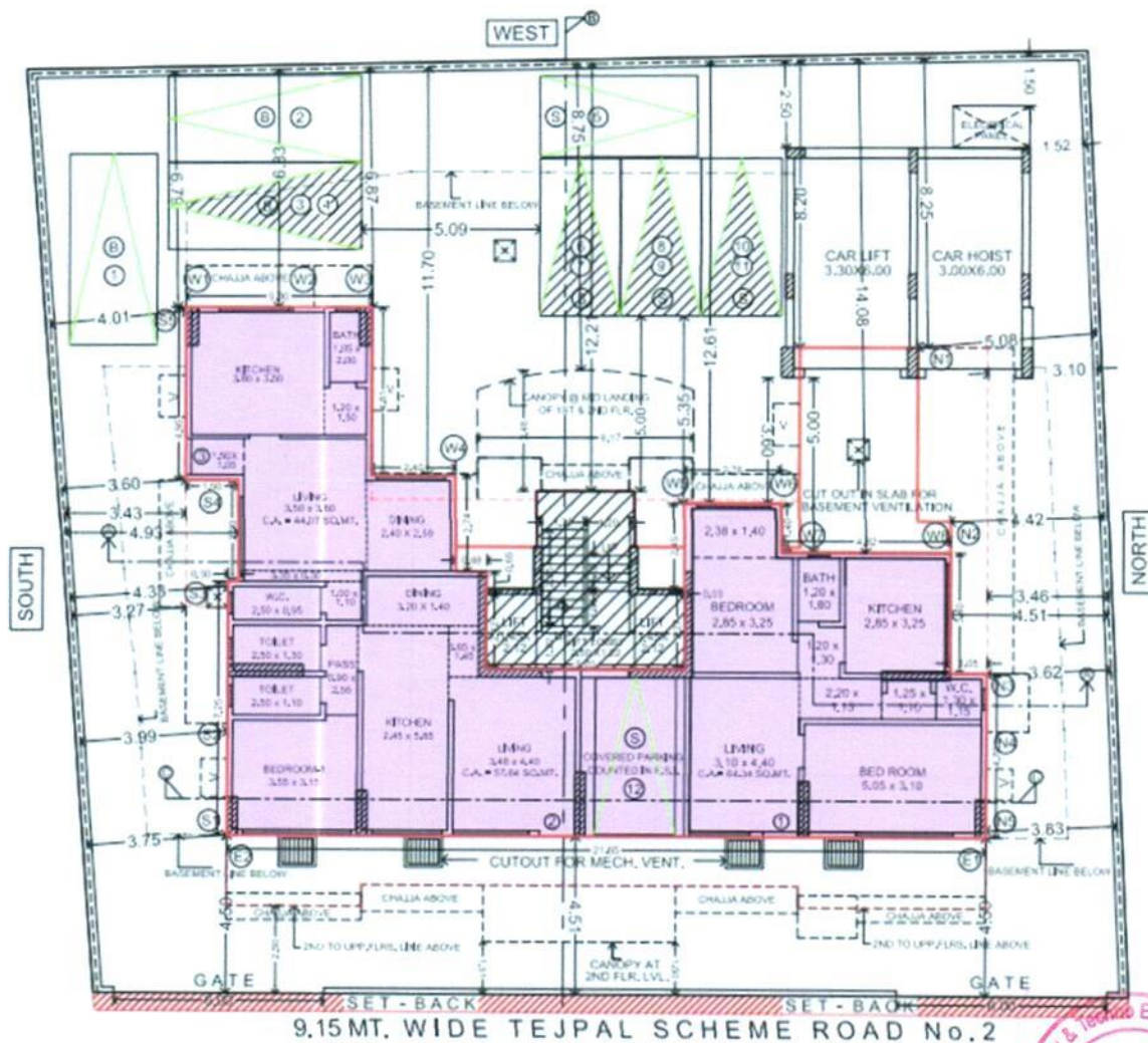
PART STILT / PART GROUND FLOOR PLAN
