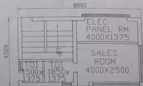
DETAILS OF U/G TANK IN MASONRY PIT UNDER RCC SLAB SCALE: NTS
