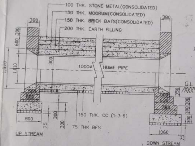
LONG SEC. OF HUME PIPE (1000Ø) CULVERT SCALE-NTS
