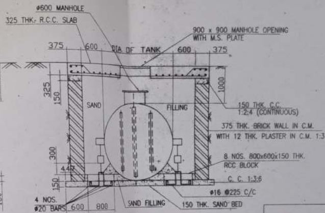
CROSS SECTION
