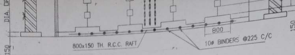
LONG SECTION
