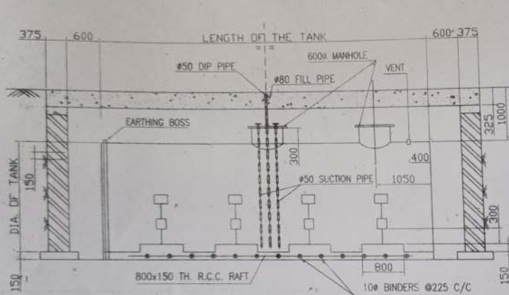
LONG SECTION
