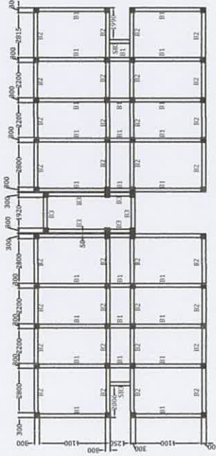
BEAM PLAN
