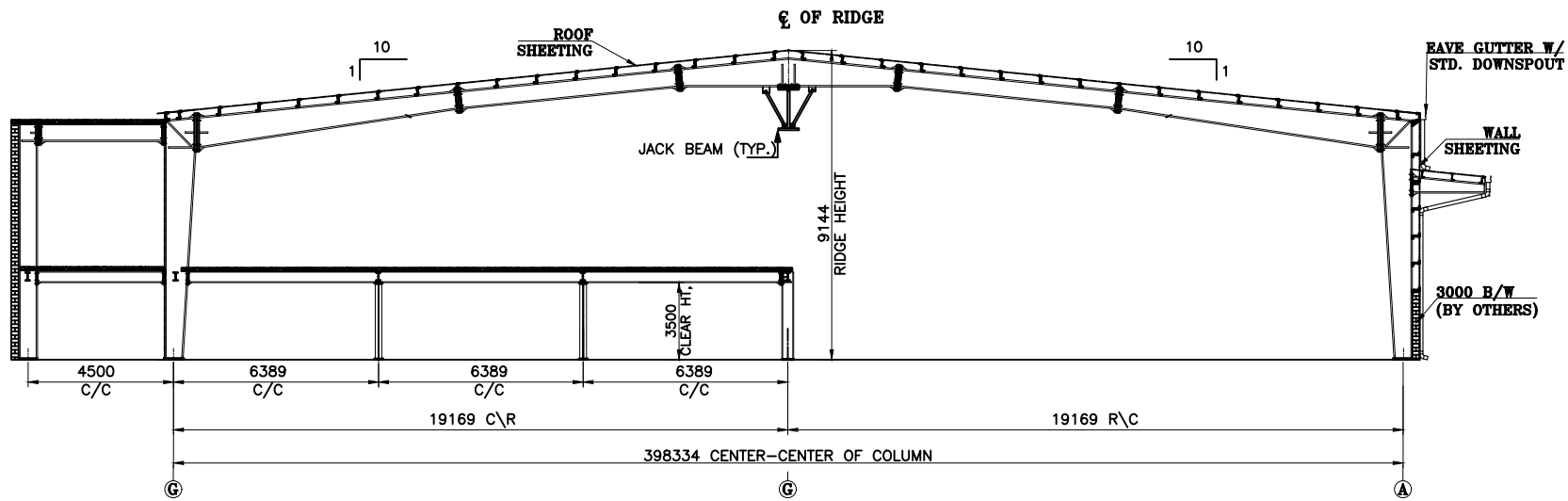
SECTION-XX
