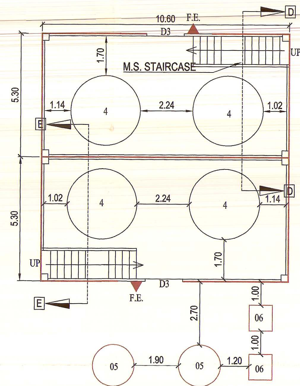
GROUND FLOOR PLAN BROMINE TANK-2
