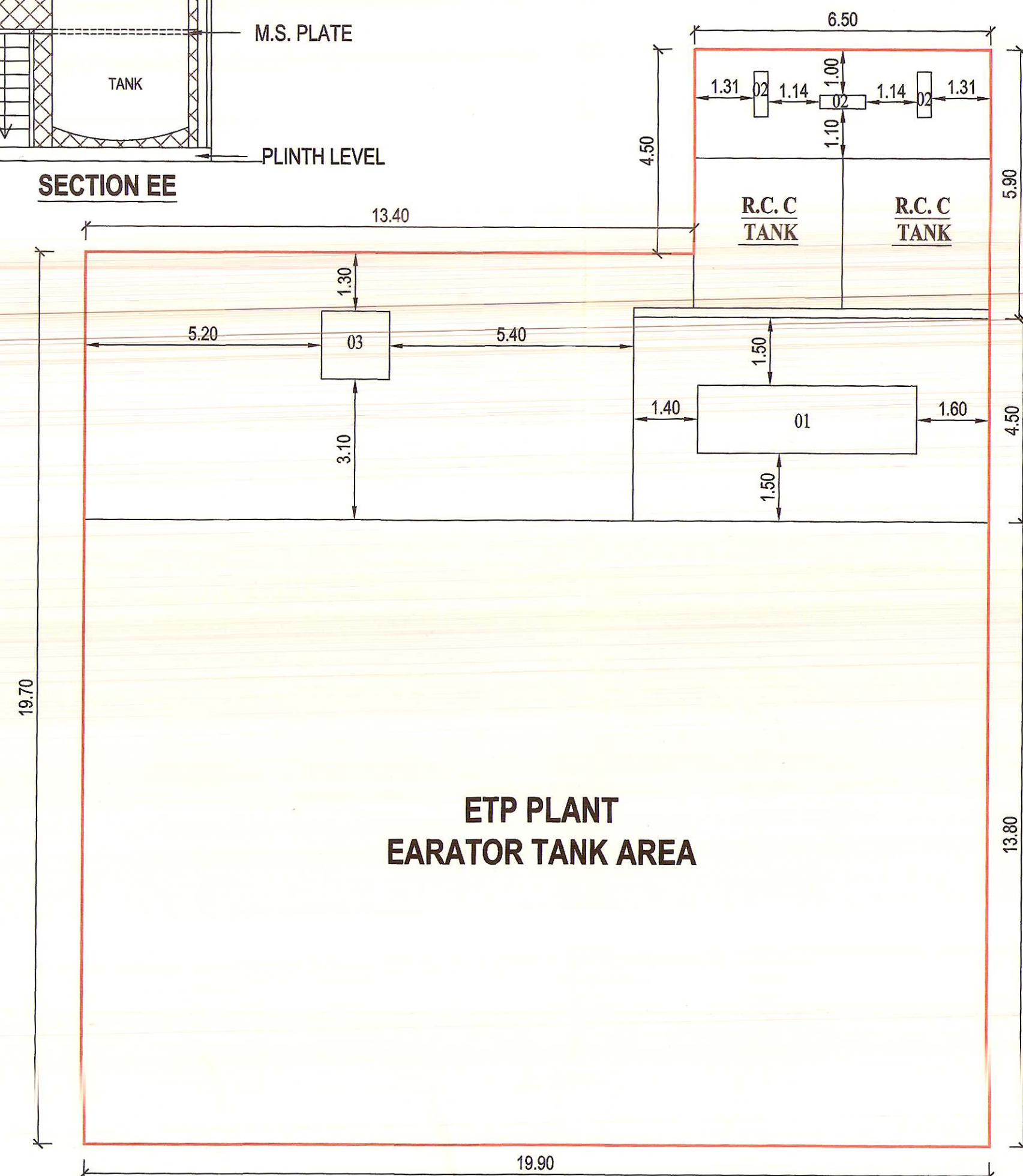
OPEN OTTA DETAILS OF ETP PLANT AREA-2
