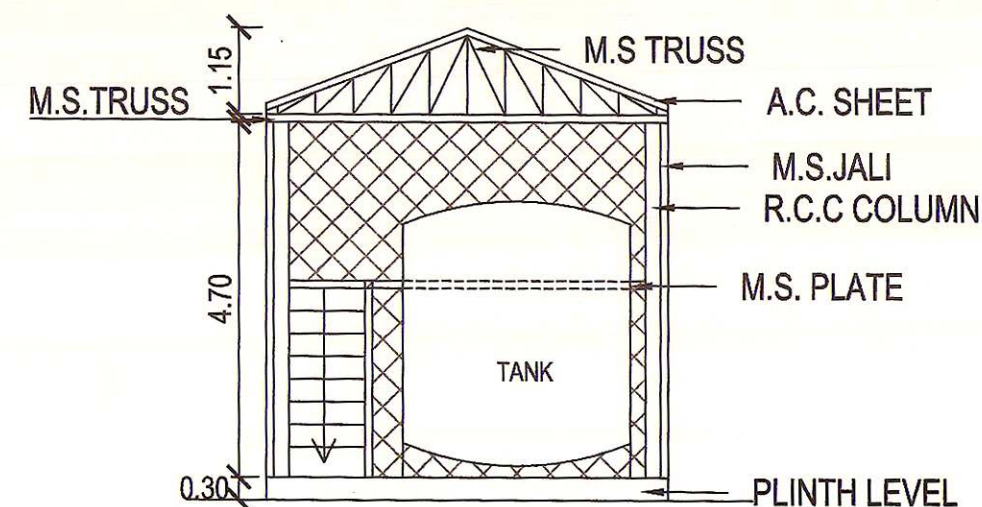
SECTION EE
