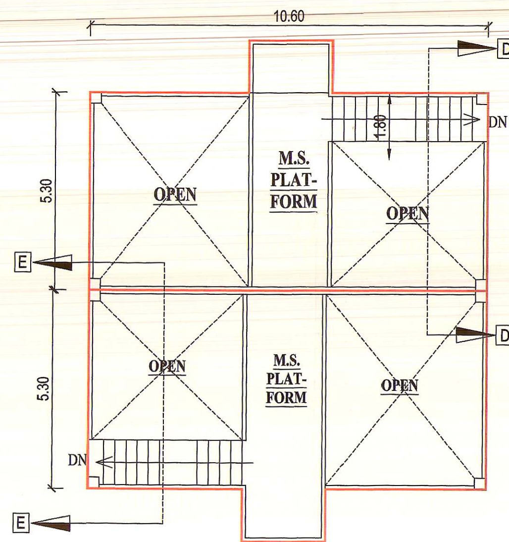
FIRST FLOOR PLAN BROMINE TANK-2
