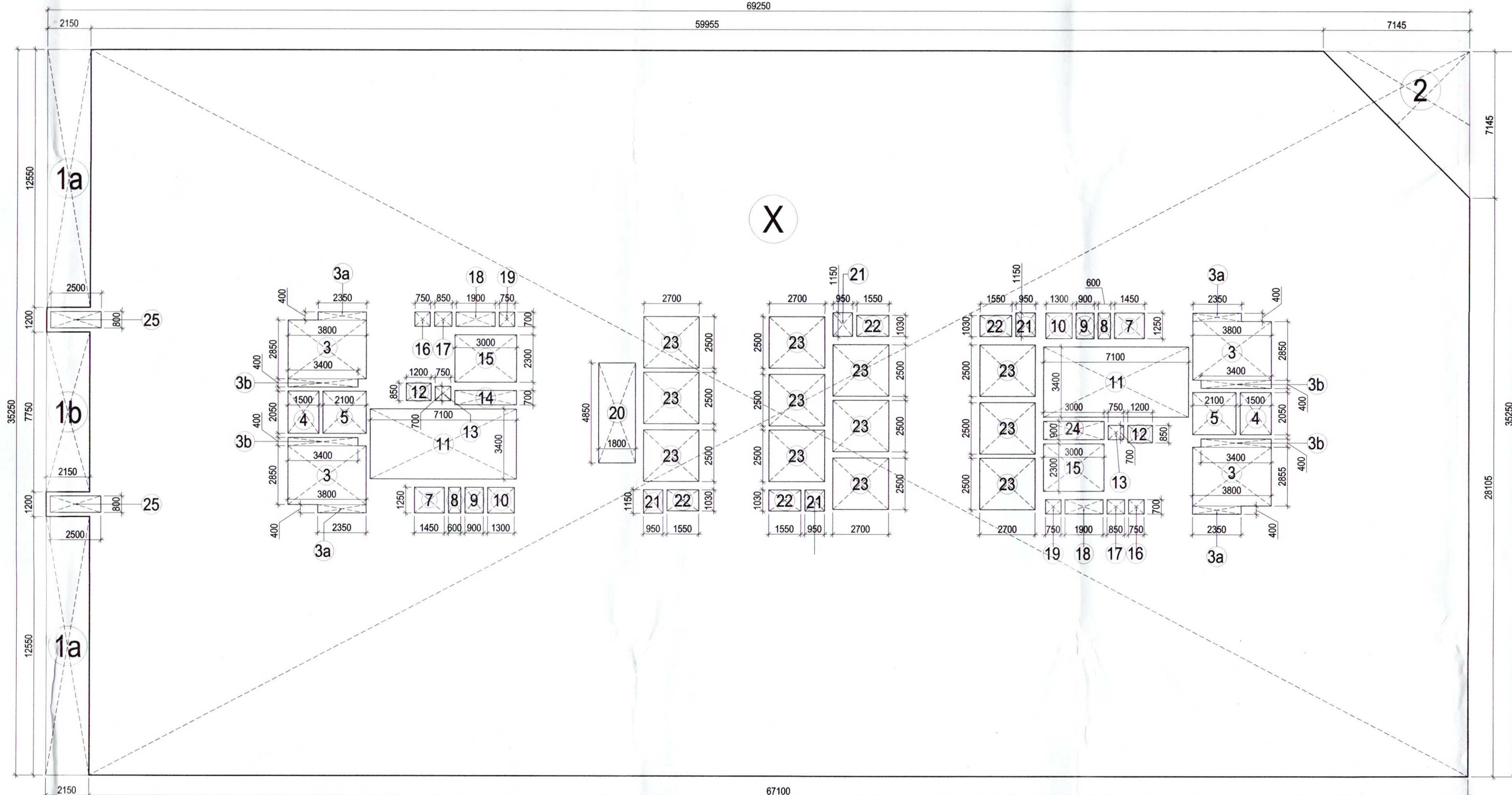
7TH FLOOR AREA DIAGRAM (TOWER_T1)
