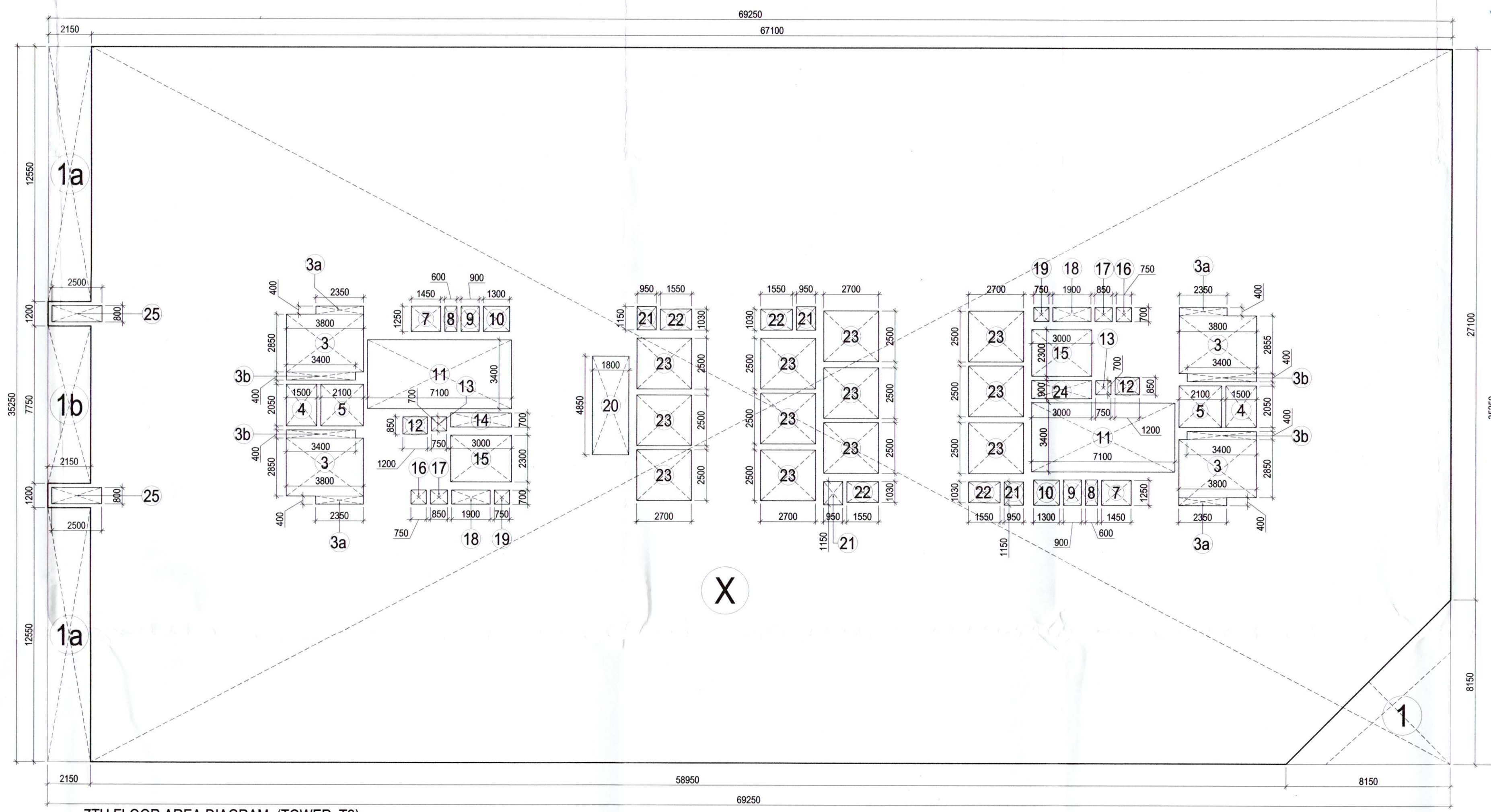
7TH FLOOR AREA DIAGRAM (TOWER_T2)
