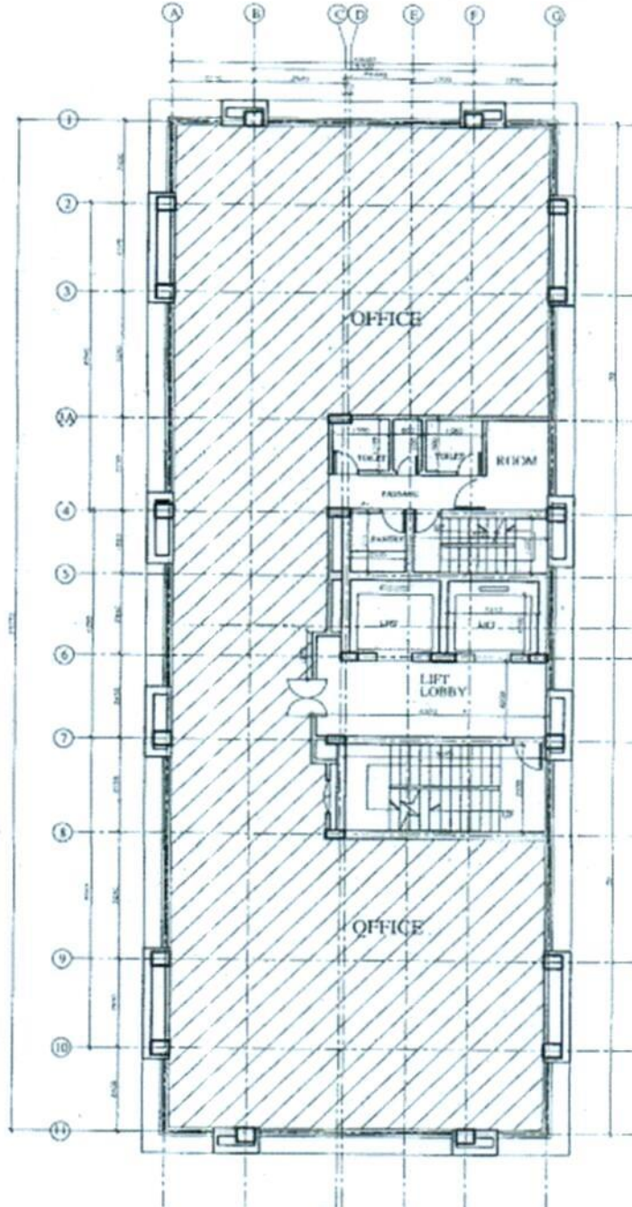
FIRST FLOOR PLAN LVL + 56.50
