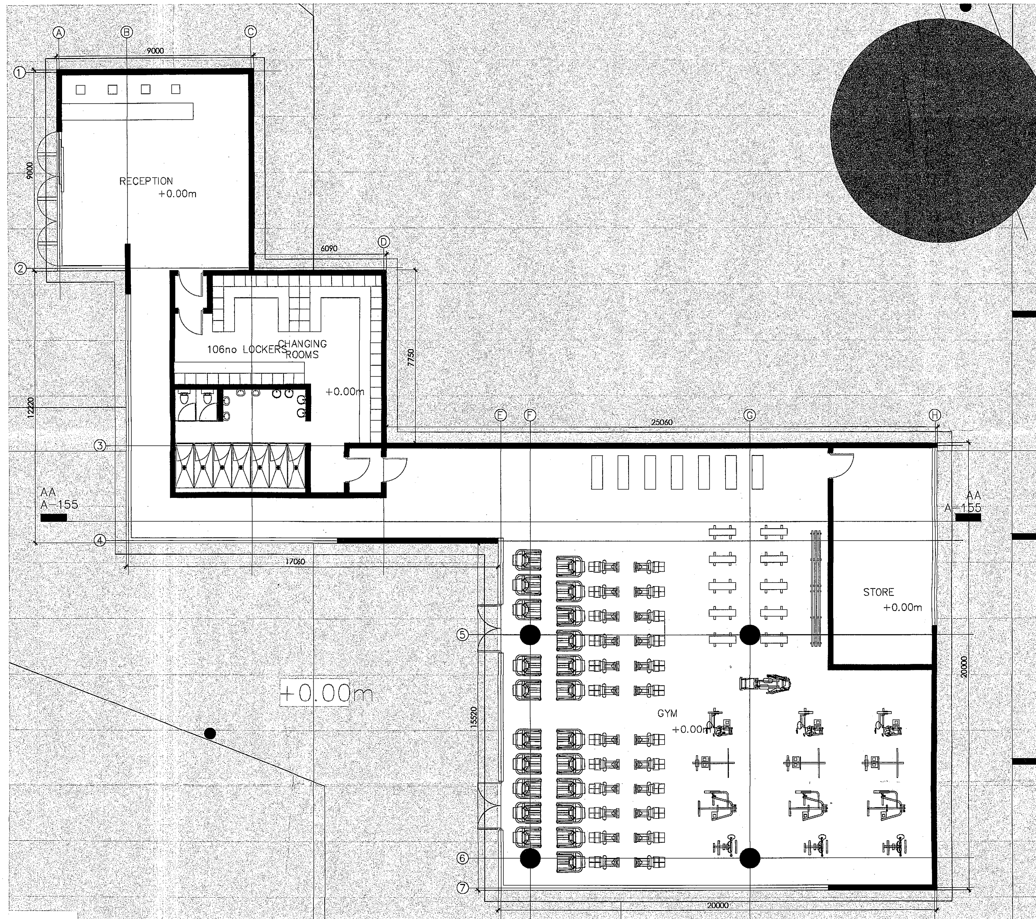
01 BOY'S HOSTEL-GYM(PHASE 1)-GF PLAN A-153 SCALE = 1:100
