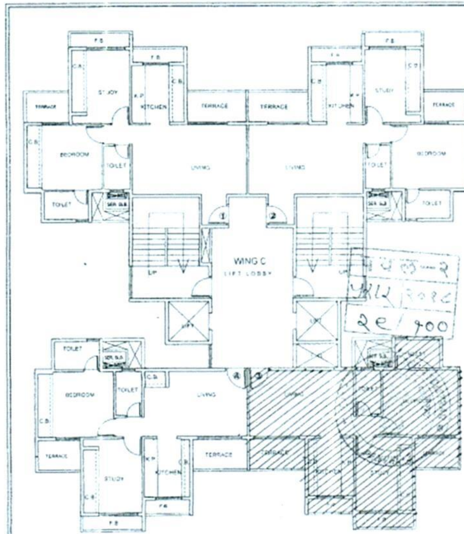
4TH, 6TH, 10TH, 12TH & 14TH FLOOR (WING - C)
