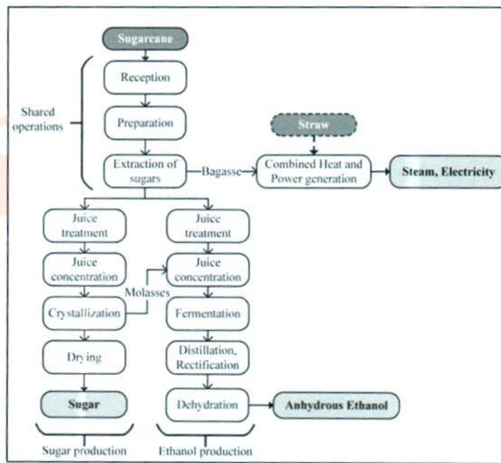
Process Cycle for Manufacturing Sugar, Ethanol & Power
