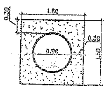
CROSS SECTION OF HUME PIPE CULVERT AT ROAD CROSSING SCALE 1:50
