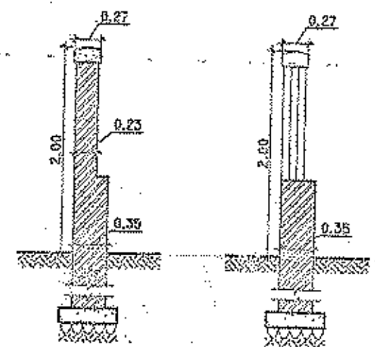
TYPICAL COMPOUND WALL DETAIL SCALE 1:50
