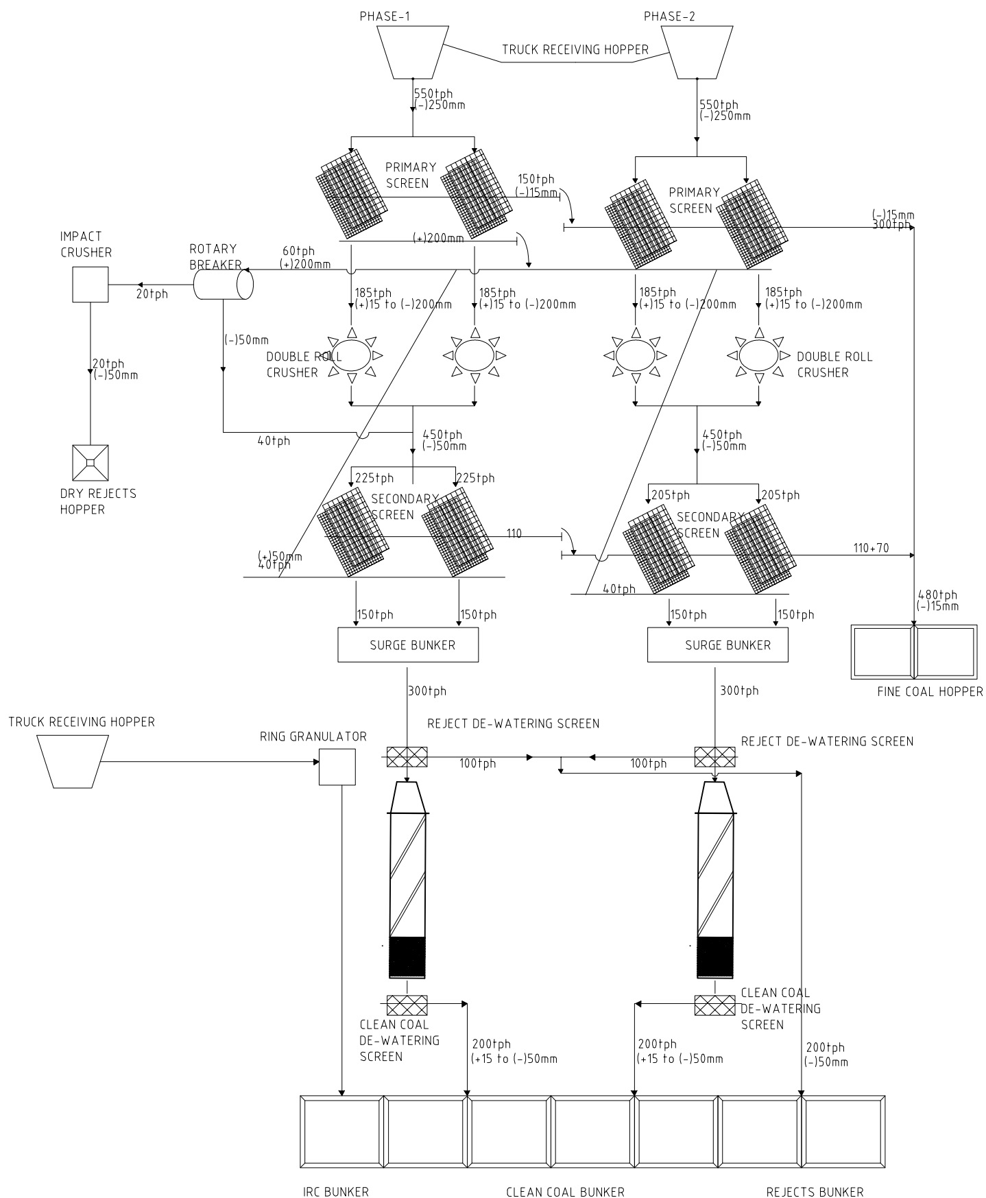
EQUIPMENT BLOCK DIAGRAM WITH MASS BALANCE
