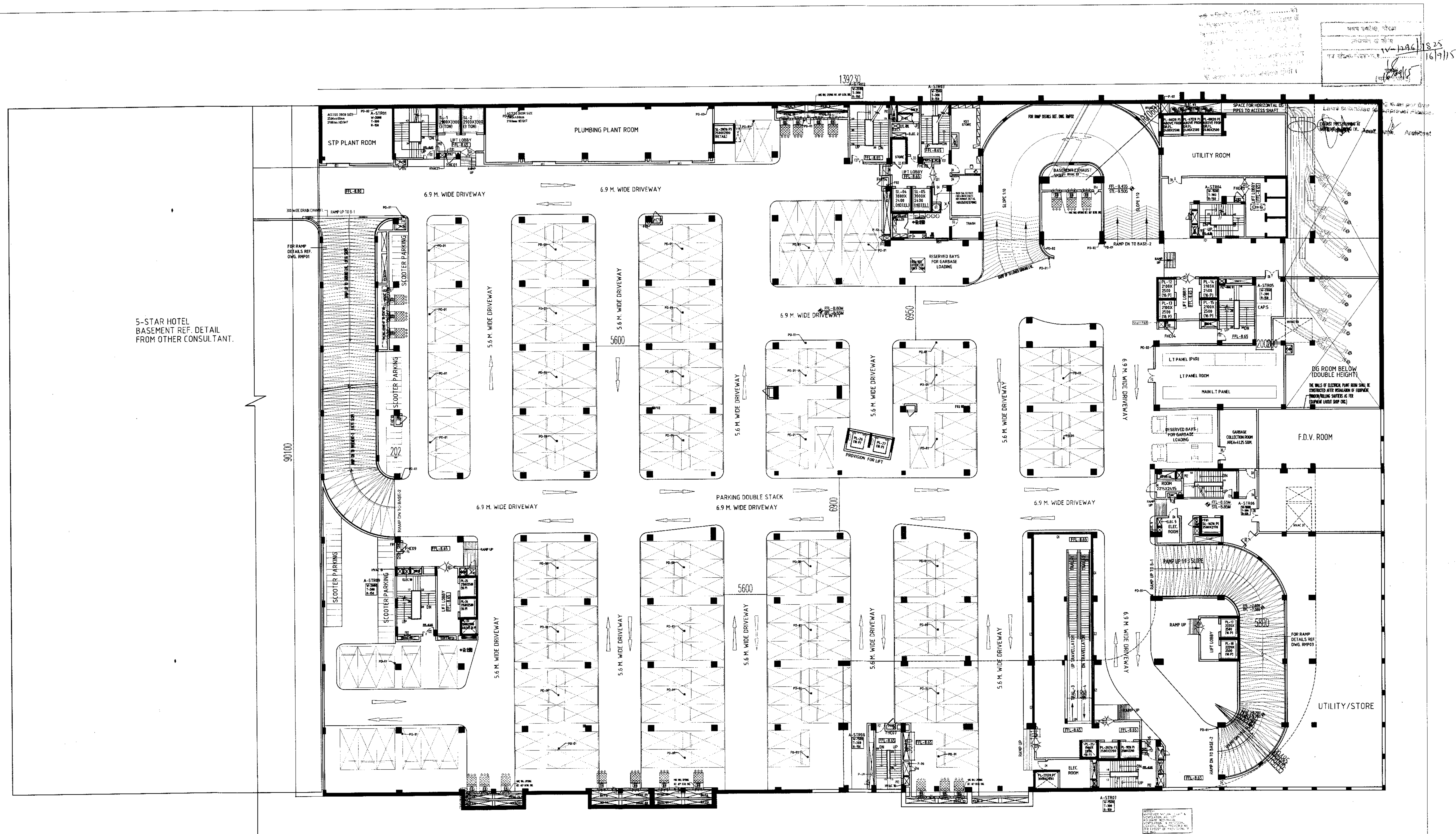
BASEMENT LVL. 2
