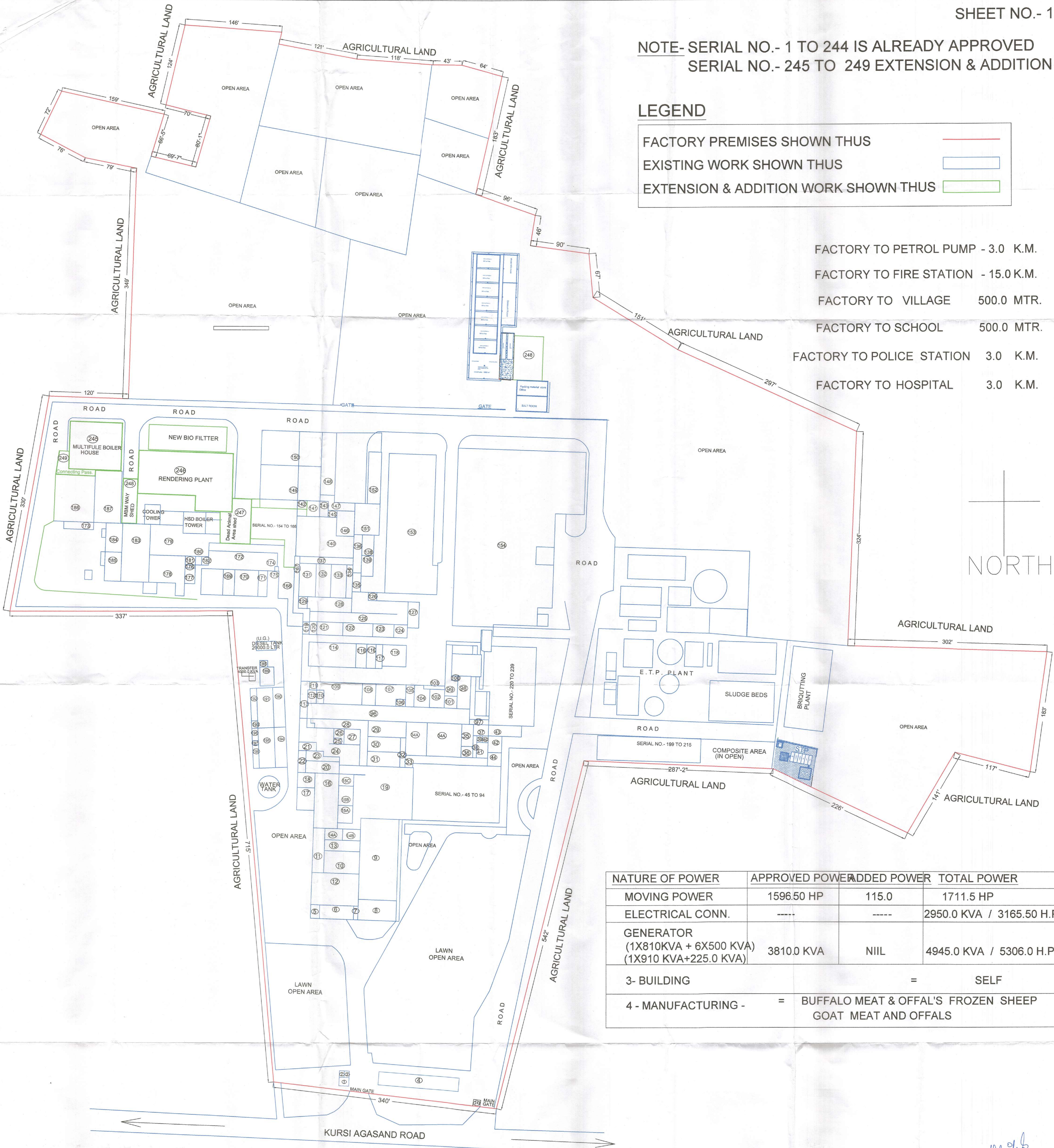
EXTENSION SITE PLAN SCALE - 1 INCH = 100 FEET
