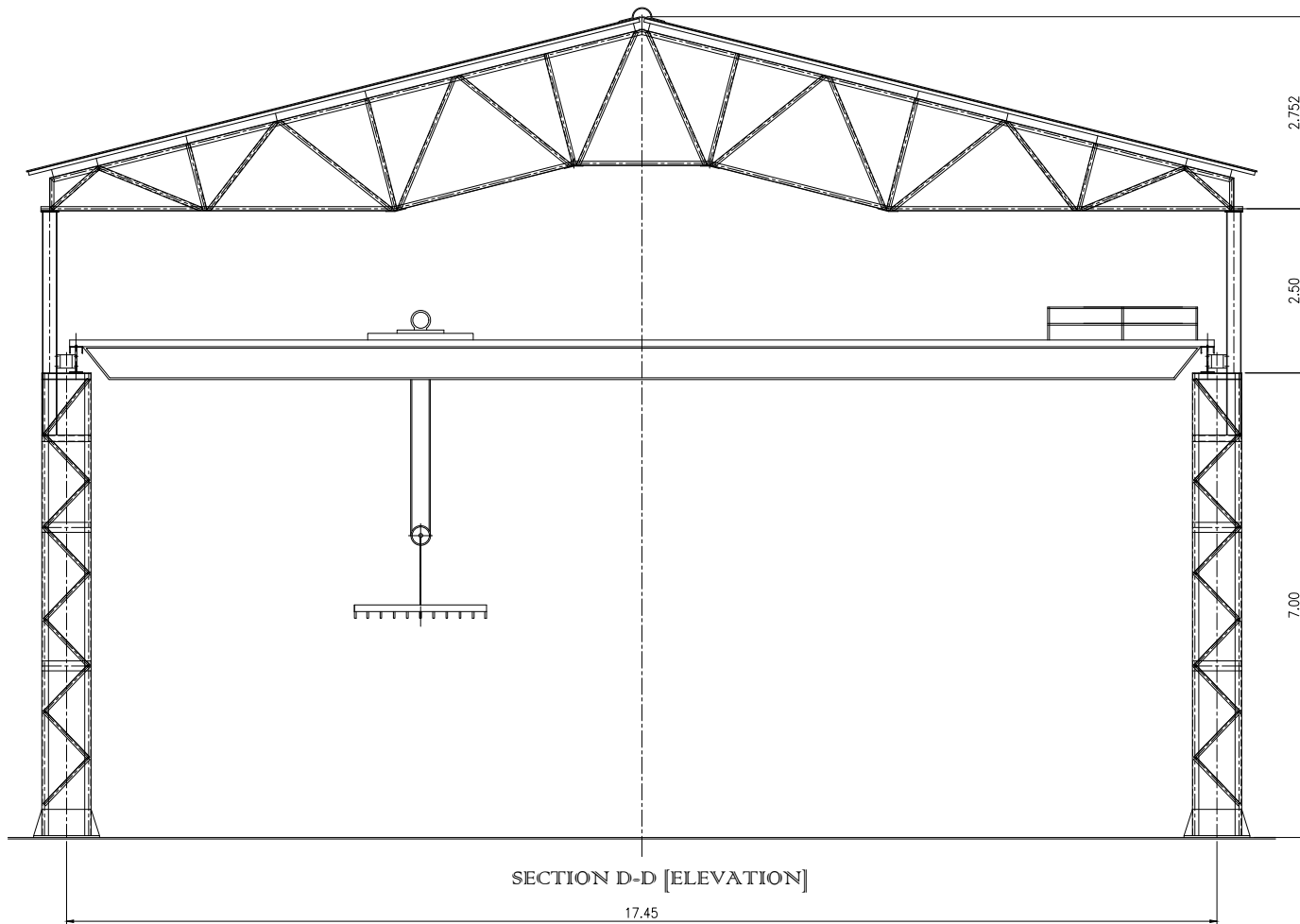
FABRICATION SHOP ( SHOP No. 2 )
