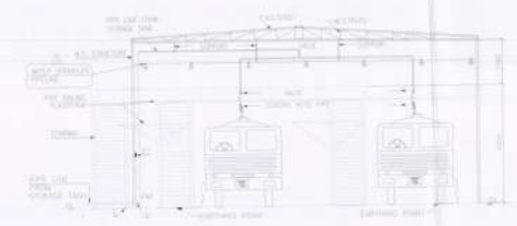
SECTION & ELEVATION OF TL LOADING PLATFORM SIZE: 18.0x12.0M SCALE: 1/80
