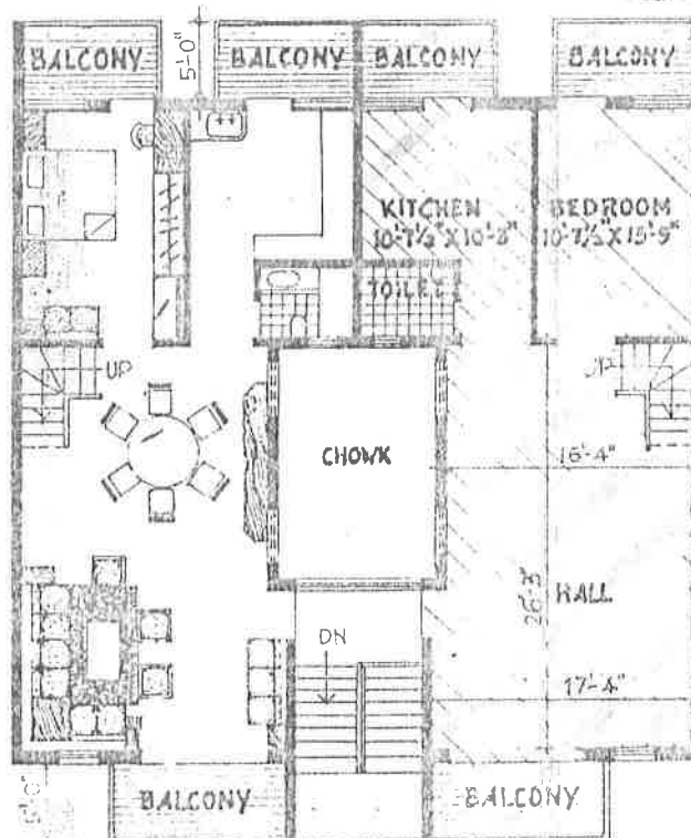
SECOND FLOOR PLAN SCALE: 1" = 12'-0"
