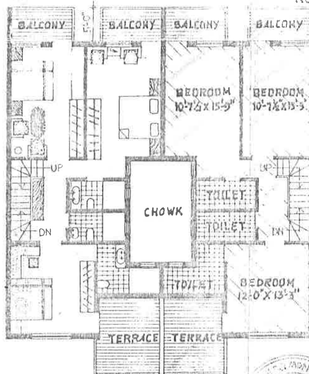
THIRD FLOOR PLAN SCALE: 1" = 12'-0"
