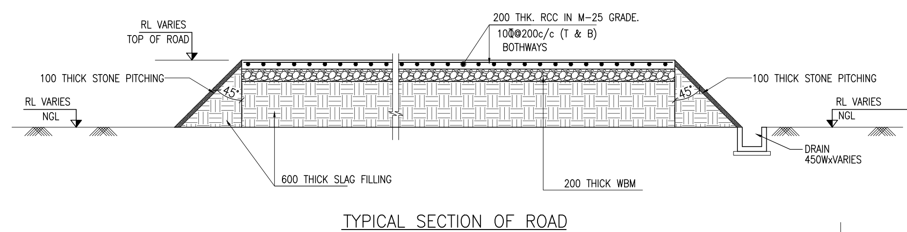
TYPICAL SECTION OF ROAD
