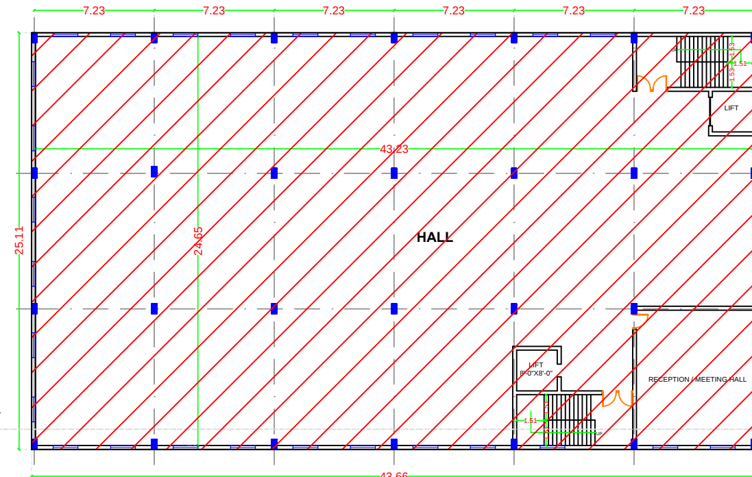
PROPOSED SECOND SERVICE FLOOR PLAN
