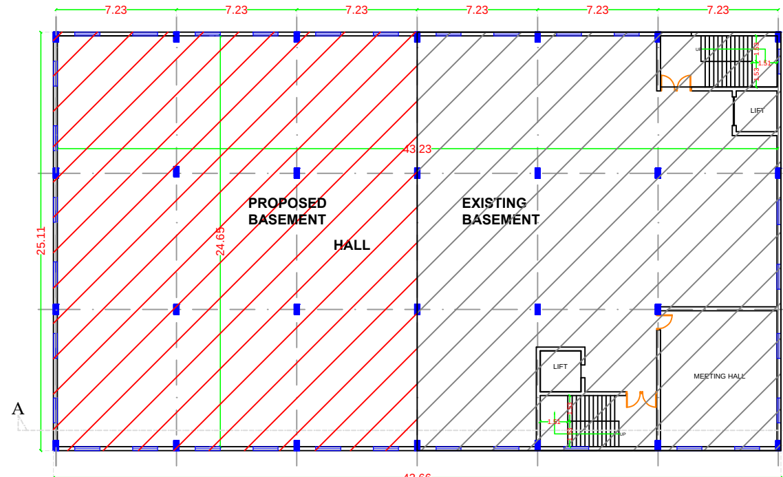
EXISTING/PROPOSED BASEMENT FLOOR PLAN
