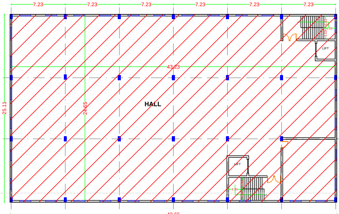
PROPOSED GROUND SERVICE FLOOR PLAN
