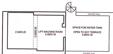
LIFT MACHINE ROOM LEVEL FLOOR PLAN
