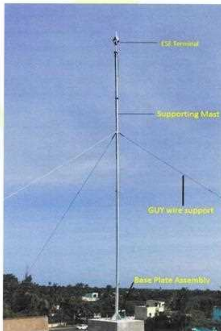
Figure 21: Illustrative image of lightning arrestor
