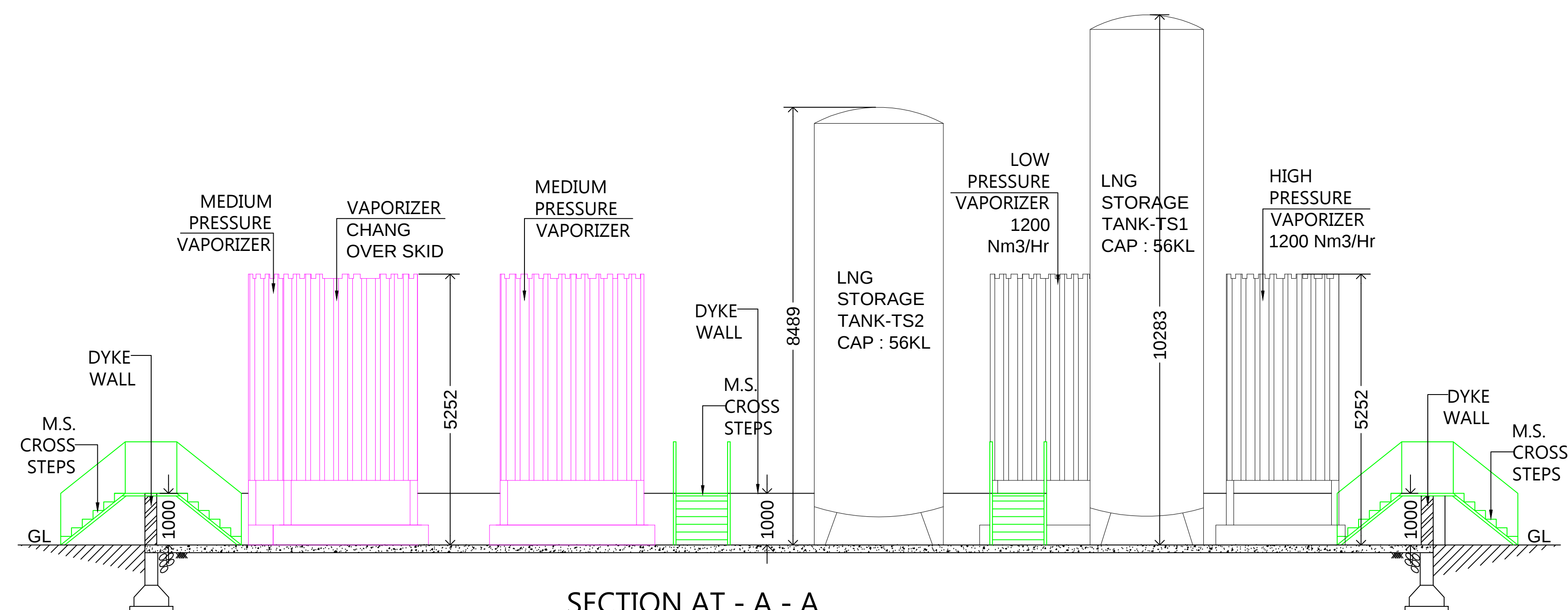
SECTION AT - A - A SCALE 1:100
