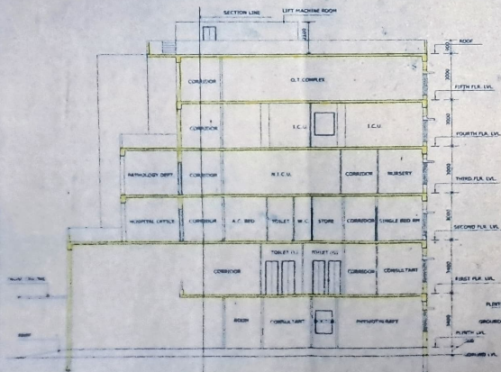
SECTIONAL ELEVATION AT A-A
