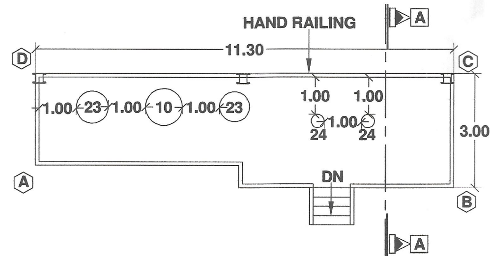
MEZZANINE FLOOR ABOVE A B C D
