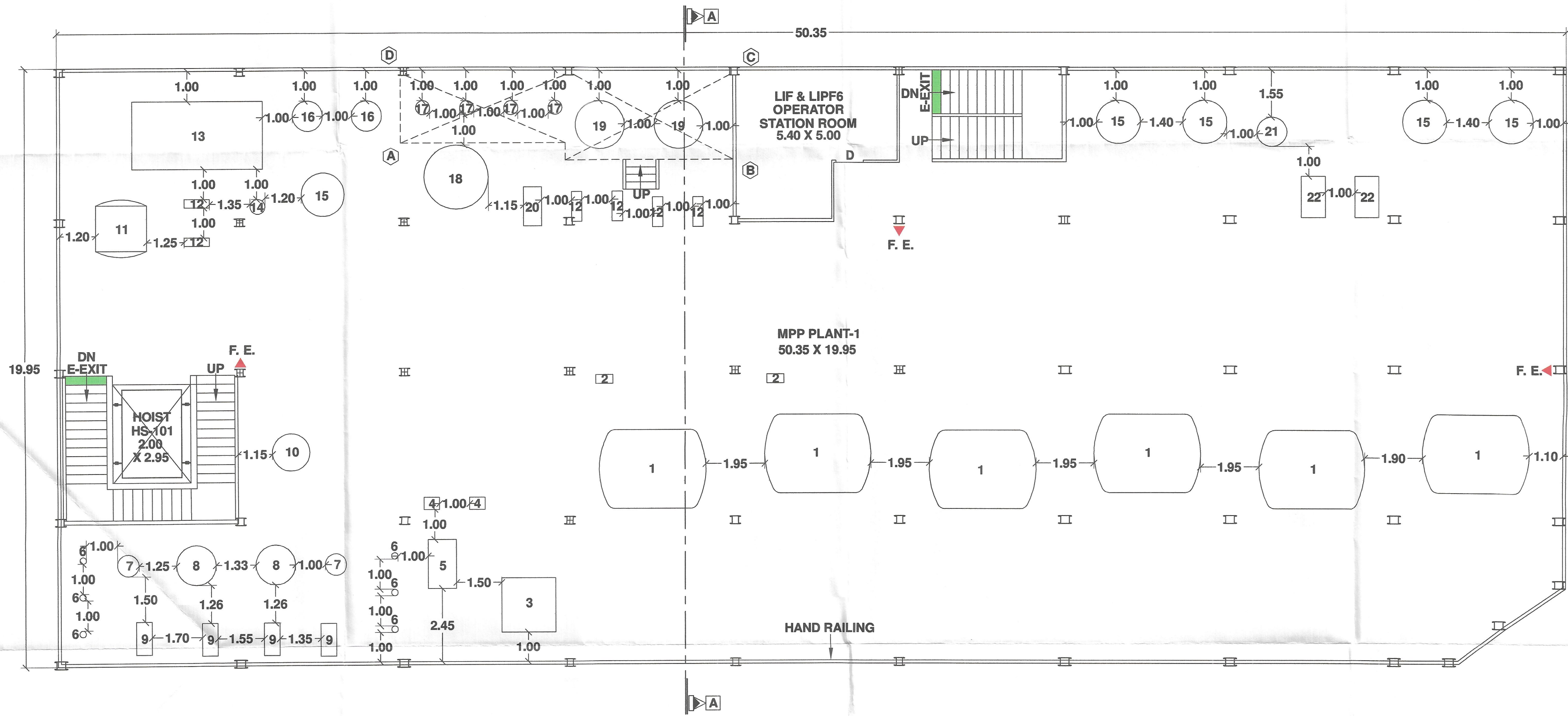
SECOND FLOOR PLAN MPP PLANT-1
